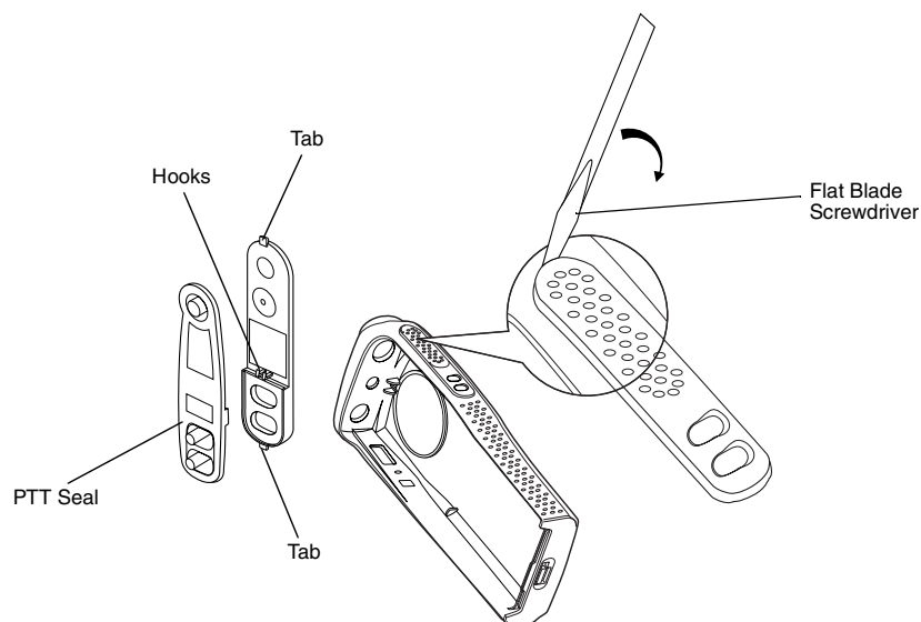
Figure 6-9. PTT Removal
