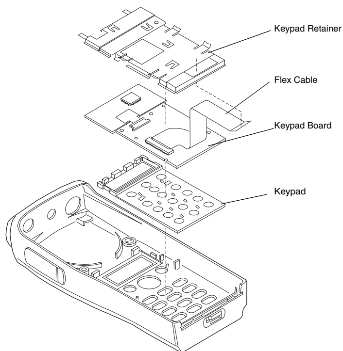
Figure 6-8. Keypad Removal
