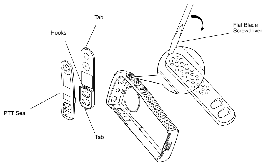
Figure 8-7. PTT Removal
