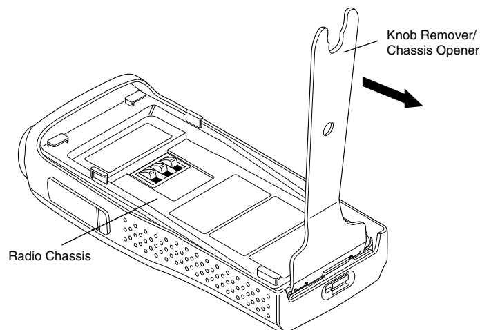
Figure 7-3. Chassis Removal
