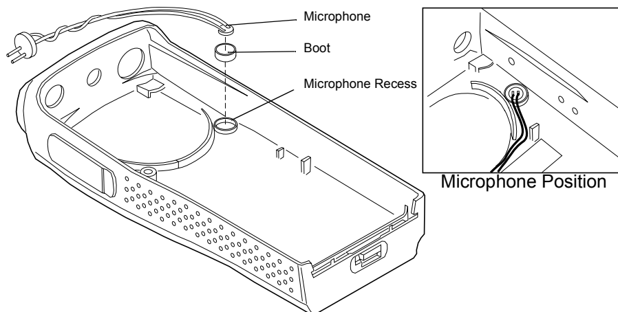
Figure 8-10. Microphone Re-assembly
