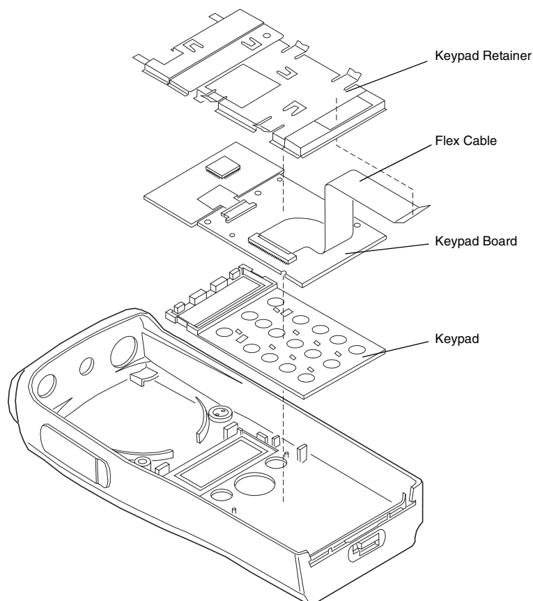
Figure 7-8. Keypad Removal
