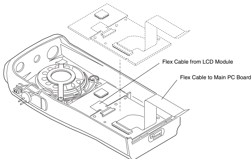
Figure 7-15. LCD/Keypad Board Re-assembly
