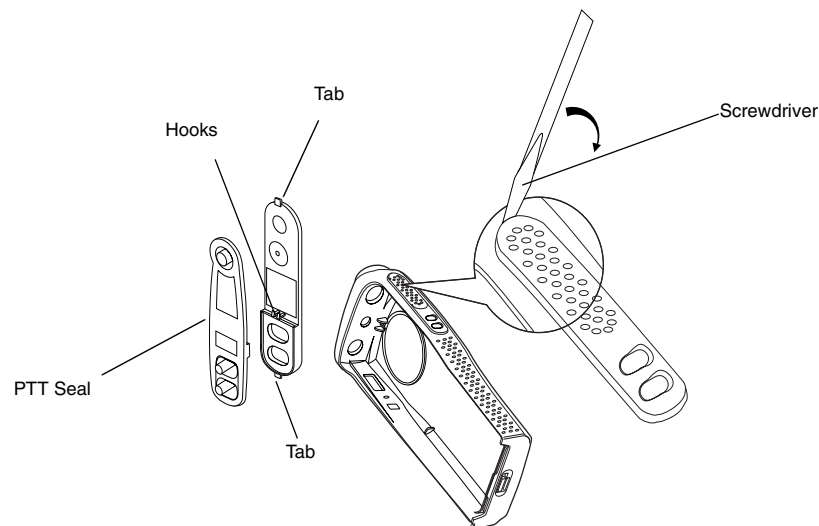
Figure 7-9. PTT Removal
