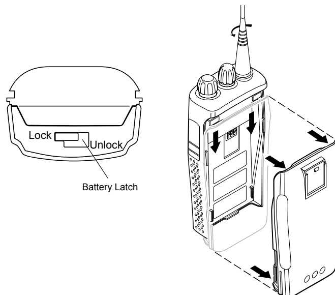
Figure 8-1. Battery Removal
