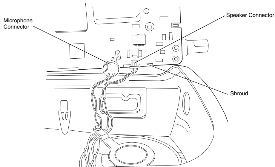
Figure 6-18. Microphone and Speaker Wires Re-assembly
